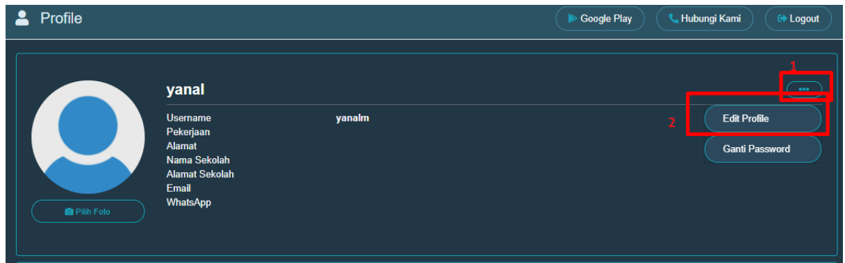
Gambar 8. Edit Profile
